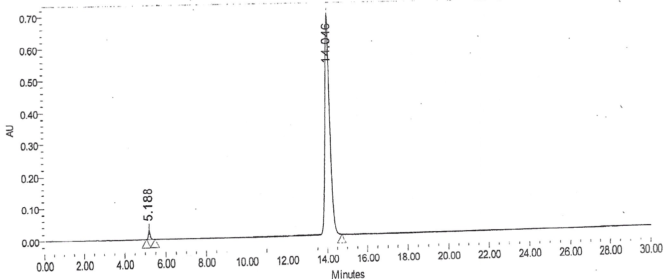
Auto-Scaled Chromatogram
